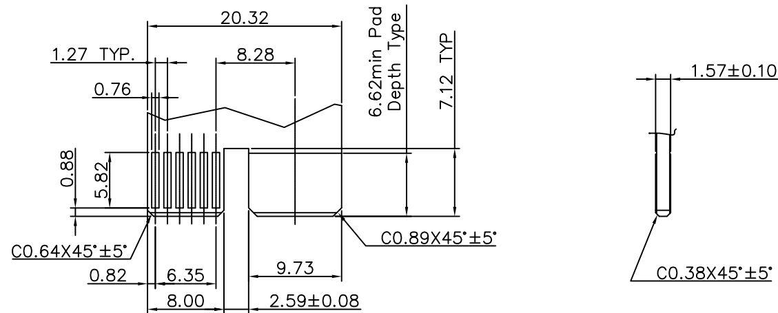
Recommended Edge Card Layout (Tolerance: ±0.05)
