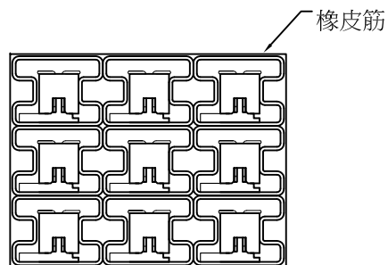
Drawing Two: Each Bundle Eight Tube (圖二: 每9管為1捆)
