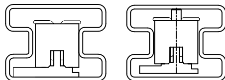
Drawing One: Product Installing Mode (圖一產品裝入方式)
