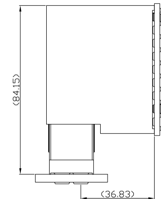
MATED PROFILE
