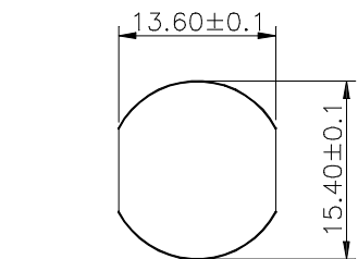
PG9 Recommended Panel CUT-Out Thickness 4.0 Max.
