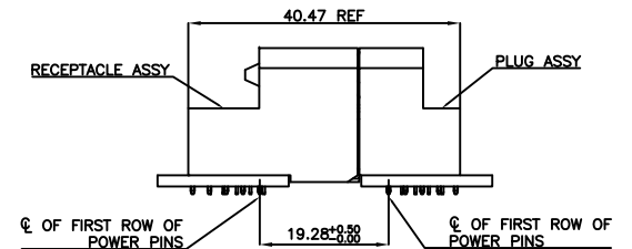
MATED PROFILE (MATED WITH R/A RECEPTACLE ASSY)
