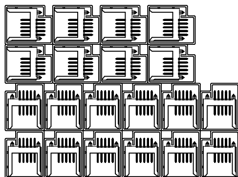
Drawing Three: Lay three bundles in each layer. Install in two layers. Five bundles, twenty tubes in all. (圖3)每層放3捆。分2層放入,一盒共5捆,共20管) Disposing schematic diagram of Tube in the inner box, for reference. (管在內盒的擺放示意圖,供參考)
